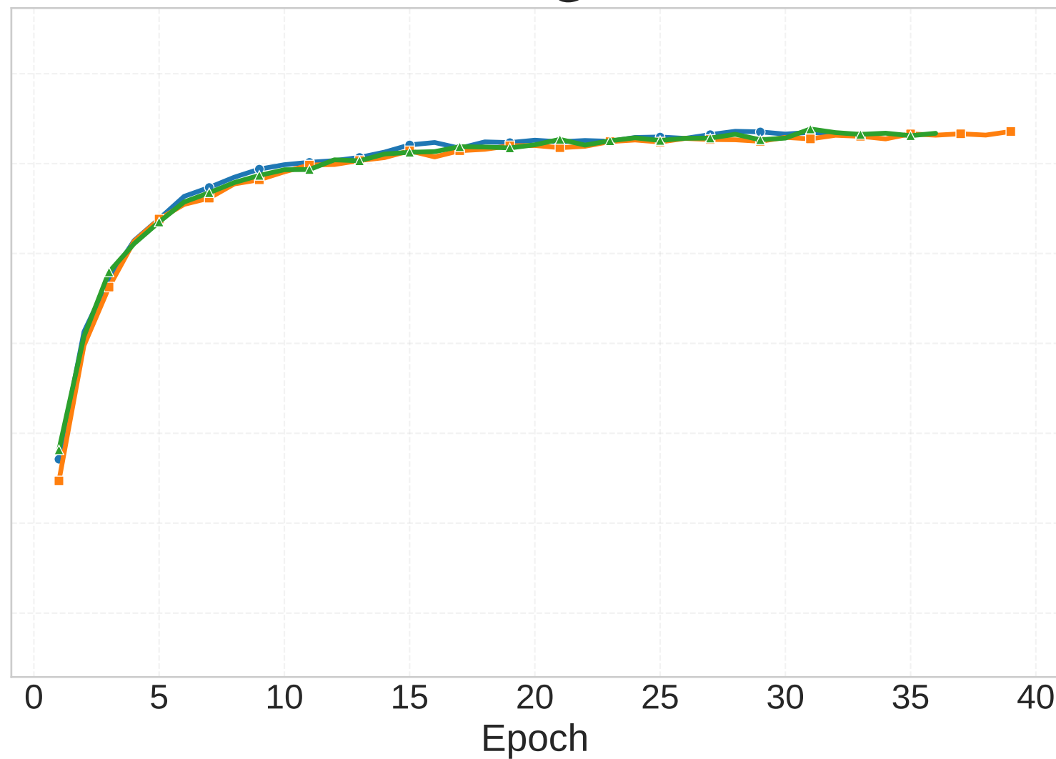
Recall @ 10
